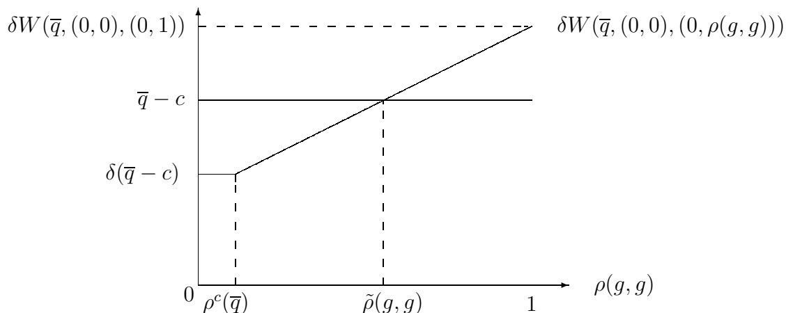
Graph 1: Existence of a MSCE in which \tilde{\rho}(g, g) \in (0, 1) .
