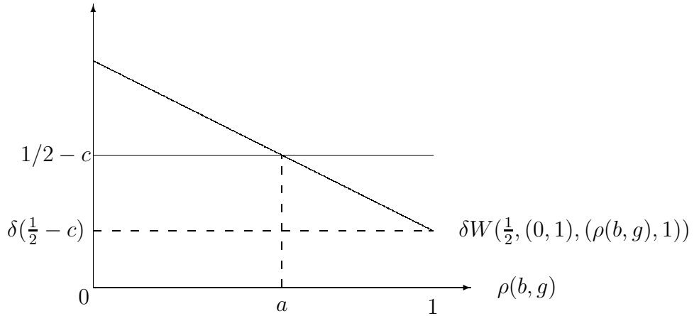
Graph 3: An unstable continuation eq. when only pessimistic receivers randomise.
